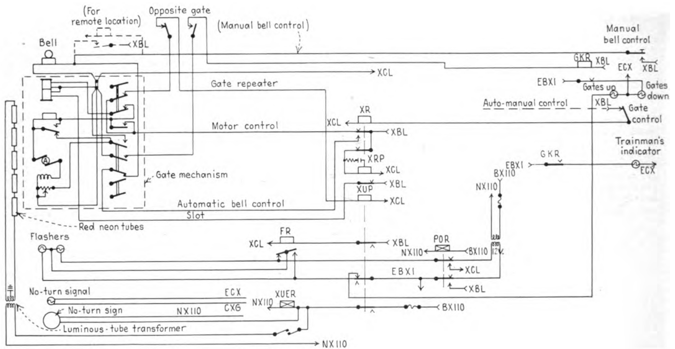
Typical neon-lighting and crossing-protection circuits
